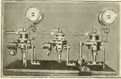
FIG. 9.—TANDEM BRAKE VALVES.
